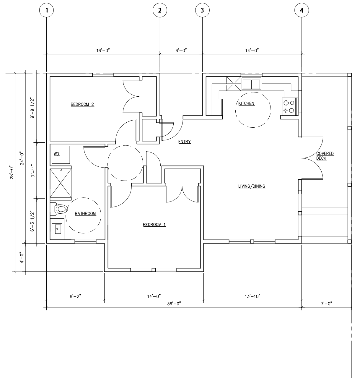
1 FIRST FLOOR PLAN A1.1 SCALE: 1/4" = 1'-0" 0' 1' 2' 4' 8'
