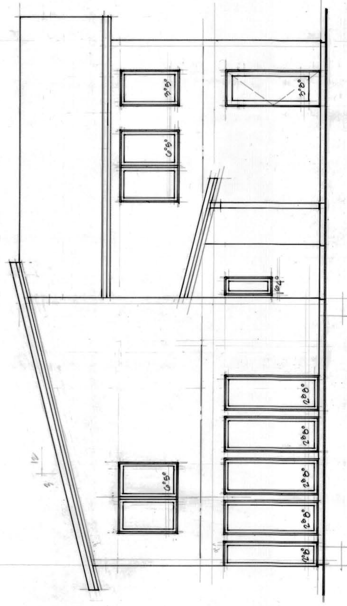
South Elevation \frac{1}{4"} = 1'-0"
